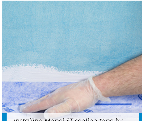
Installing Mapei ST sealing tape by using Mapegum WPS, floor/wall transition
